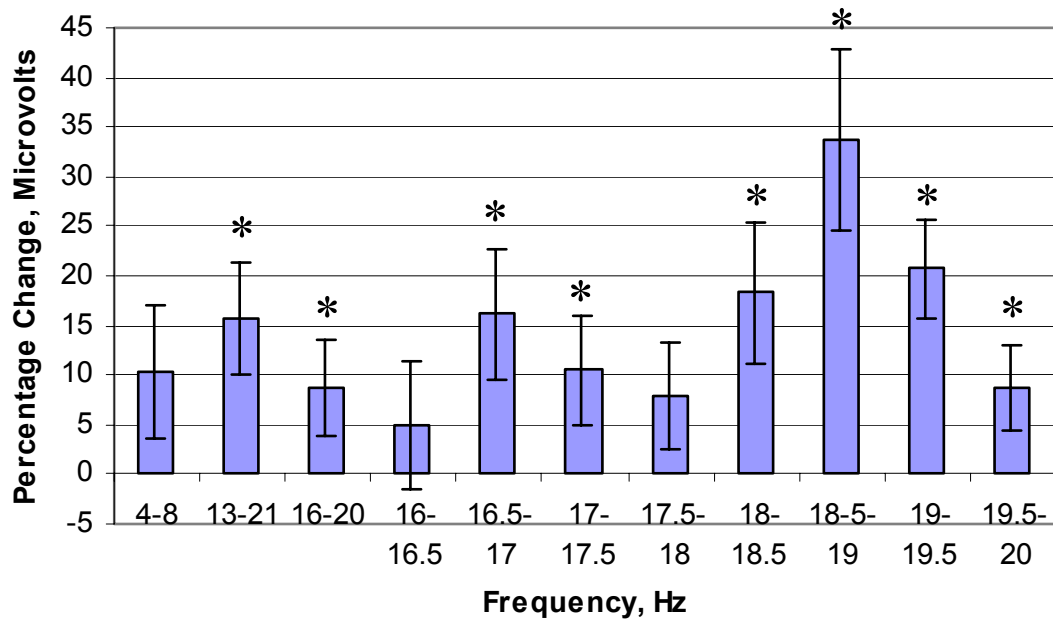
Fig. 1. Effect of 18.5 Hz Auditory and Visual Stimulation on EEG Amplitude at the Vertex (All Conditions Combined)
